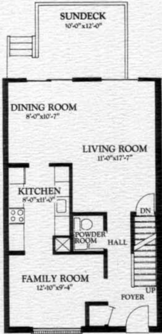
FIRST FLOOR WITH SUNDECK
