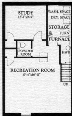
OPTIONAL FINISHED BASEMENT Front Recreation Room Non-Walkout
